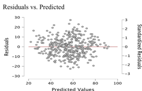
Figure 2. Heteroscedasticity Test
